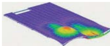
Finite element model showing the first mode of vibration for the first floor at the SCI headquarters
